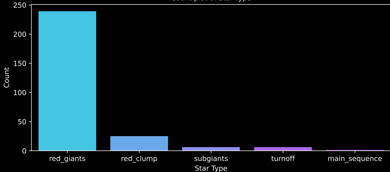
APOGEE DR17 Field: [326+06] Count plot of Star Type
