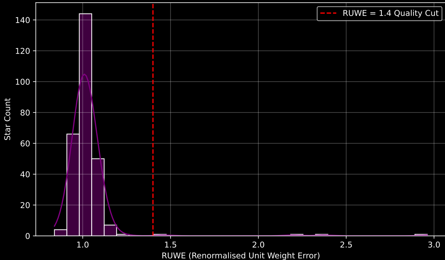
GAPOGEE DR17 Field [326+06] RUWE Distribution (n= 276)
