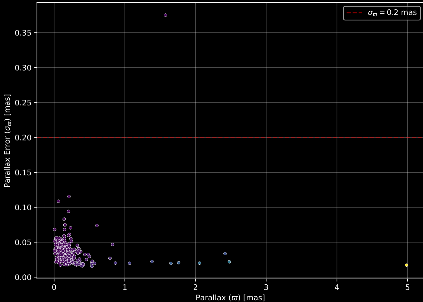
APOGEE DR17 Field: [326+06] Parallax Quality (n= 277)
