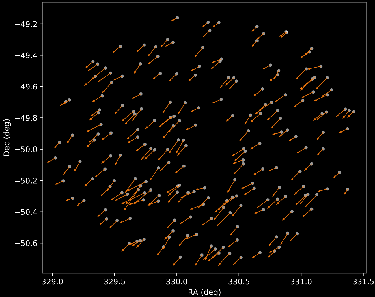
APOGEE DR17 Cluster 2 Proper Motion Vectors (n=202)
