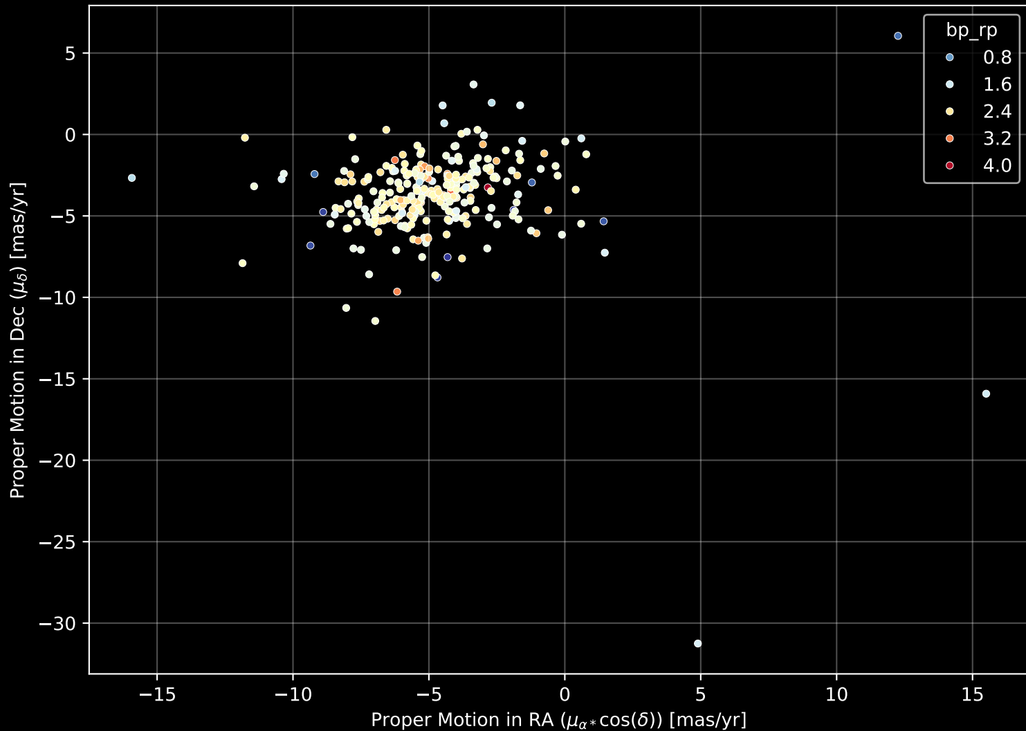
APOGEE DR17 Field: [326+06] Proper Motion Diagram (n= 277)
