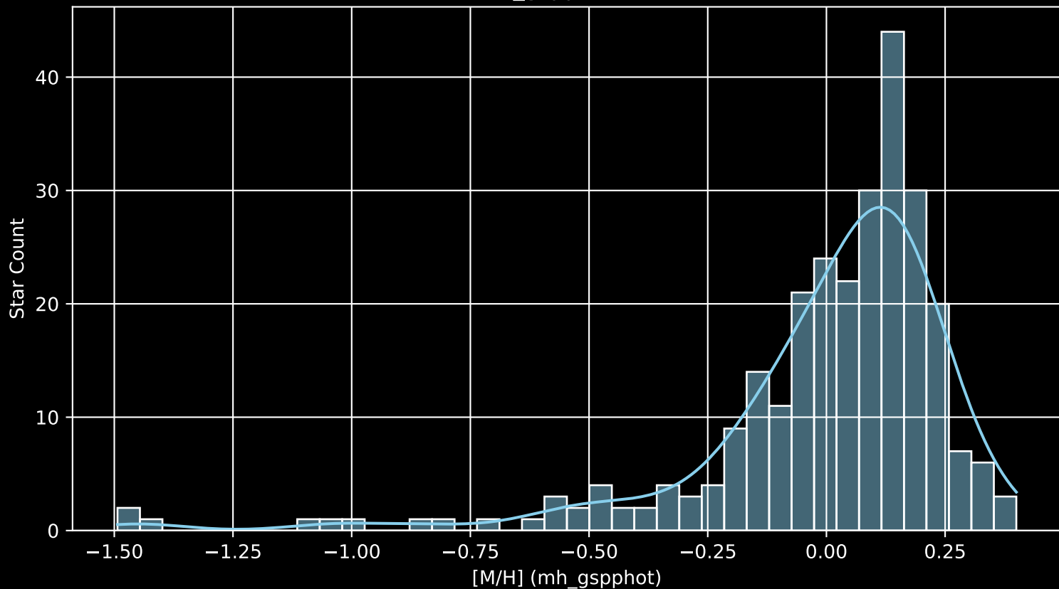
APOGEE DR17 Field: [326+06 [M/H] (mh_gspphot) (n= 275)
